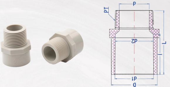
外牙直接 MALE ADAPTER
