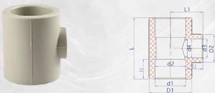
异三通 REDUCER TEE
